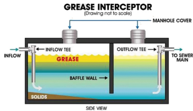
Grease Interceptor
